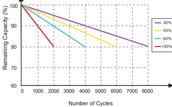
CYCLE LIFE vs.DEPTH OF DISCHARGE(DOD) DISCHARGE@1C, 25°C
